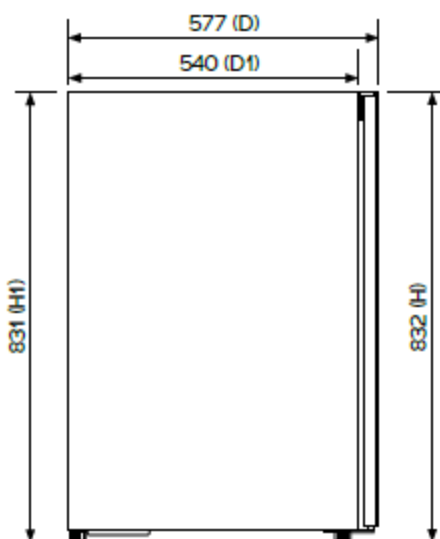
PROFILE VIEW
