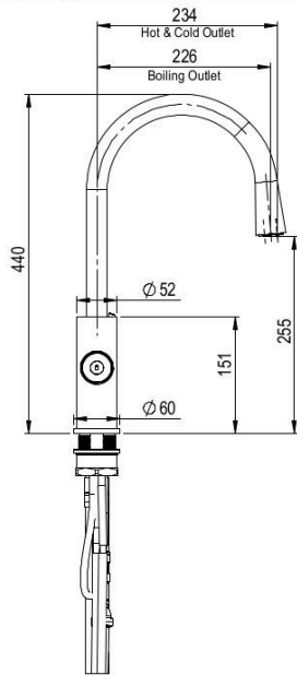
LHS VIEW
