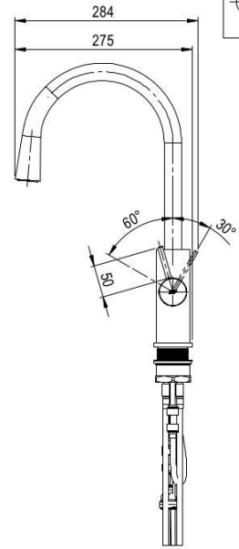
RHS VIEW
